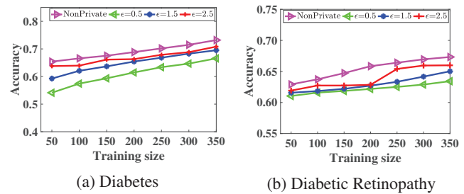
Figure 6: The classification accuracy of OffPairC for metric learning task under different training sizes.
