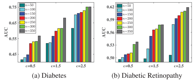
Figure 4: The AUC measurement of OffPairC.
